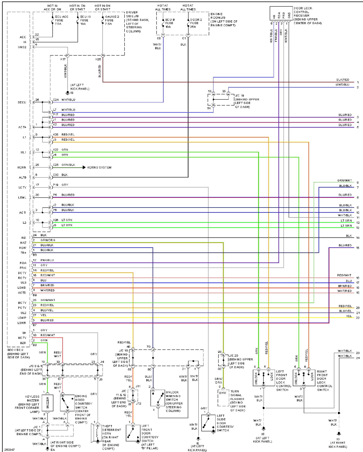
Fig. 55: Power Door Locks Circuit (1 of 2)
