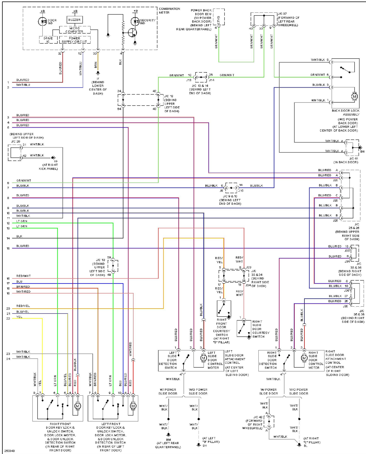
Fig. 56: Power Door Locks Circuit (2 of 2)
