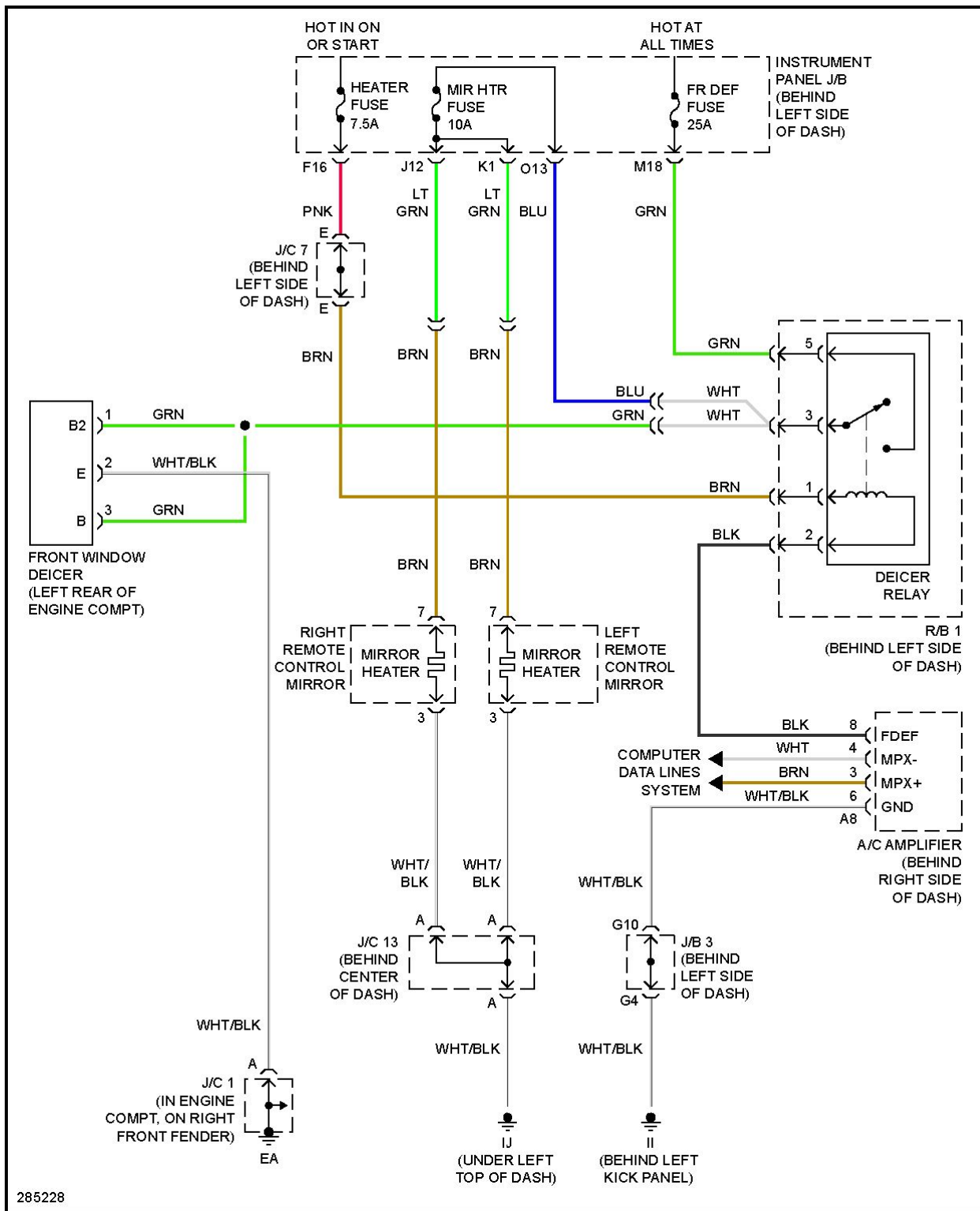
Fig. 17: Heated Mirrors Circuit, W/O Memory
